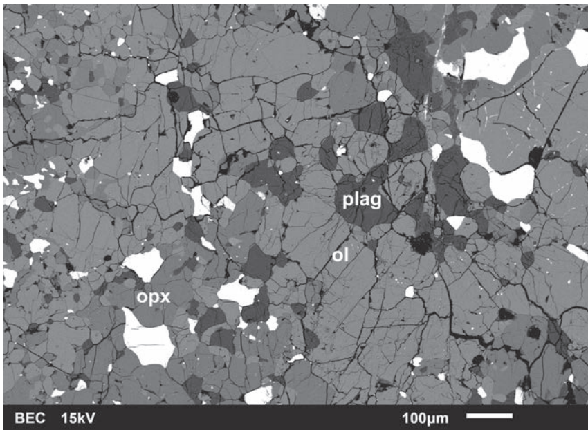
Fig. 5. BSE image exhibiting the strongly recrystallized lithology, consisting mainly of olivine (light grey), orthopyroxene (medium grey), plagioclase (dark grey), and anhedronal grains of metal and troilite (white).
