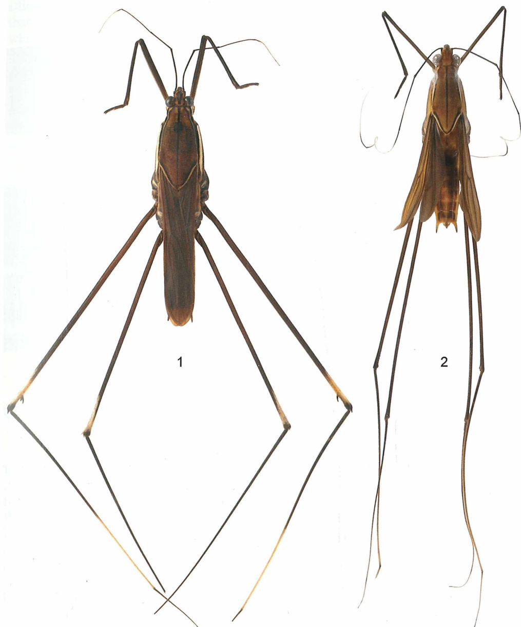
Figs. 1–2: Dorsal aspects of (1) Limnometra freitagii sp.n., ♂, holotype; (2) Limnometra tiomansensis sp.n., ♂, paratype.
