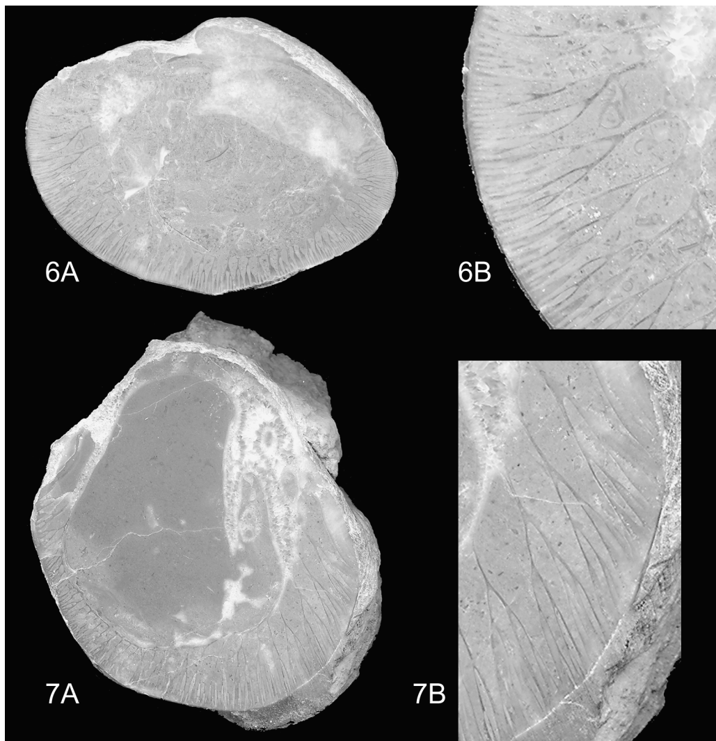
Fig. 6, 7: Plagiptychus aguilloni (d'ORBIGNY, 1840) from (6) Lupat, near Grünbach, NHMW 2004z0078/0001, (7) Grünbach, Pfarrer Schweighofer, NHMW 2004z0078/0002. (A) Adapical views of LV, x1,05. (B) Details of posterior inner shell wall with pallial canals.
