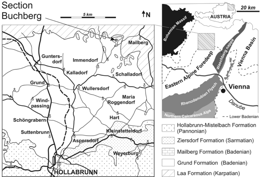
Fig. 1: Geological setting of the studied section. The study area is part of the north-eastern part of the Alpine Molasse Basin. The carbonates and marls of the Mailberg Formation interfinger with the topmost part of the open marine siliciclastics of the Grund Formation. The map on the left combines regional geology and lithostratigraphy of ROETZEL & PERVESLER (2004) with the topography of the Austrian Map 1:200,000 (BEV, Vienna). The map on the right with the geotectonic setting of north-eastern Austria is modified after RÖGL & SPEZZAFERRI (2003); the distribution of Lower Badenian sediments follows PAPP et al. (1978).
