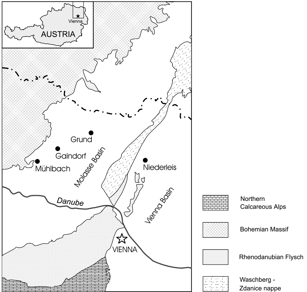
Fig. 1: Generalized tectonic map with the position of the localities Mühlbach, Gaidorf and Grund.
