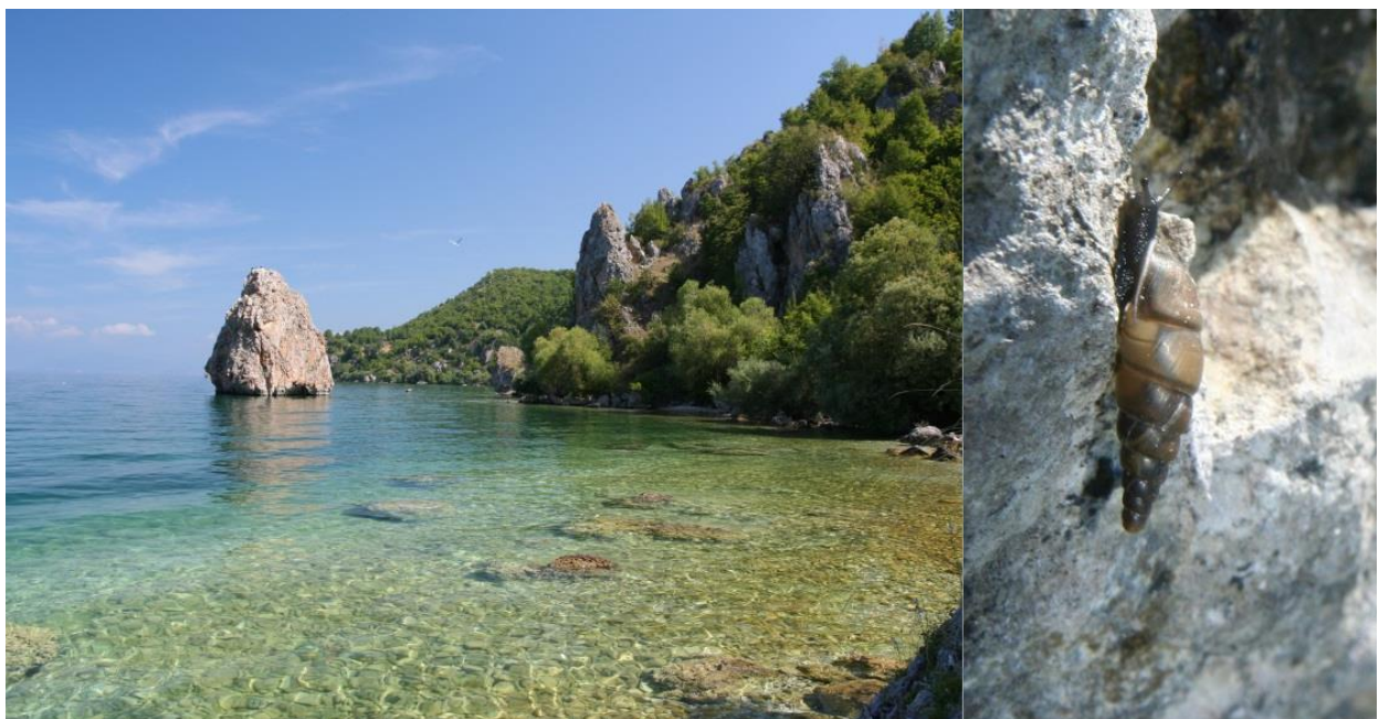
Figure 13. Cliffs along the shore of Lake Ohrid, north of Trpejca, Macedonia. This is one of the known sites where two different Montenegrina species can be found at the same locality. M. stankovici (on the right) prefers the lowest regions directly above the water surface, while M. dofleini pinteri inhabits higher parts of the same cliff; © Z. Feher
