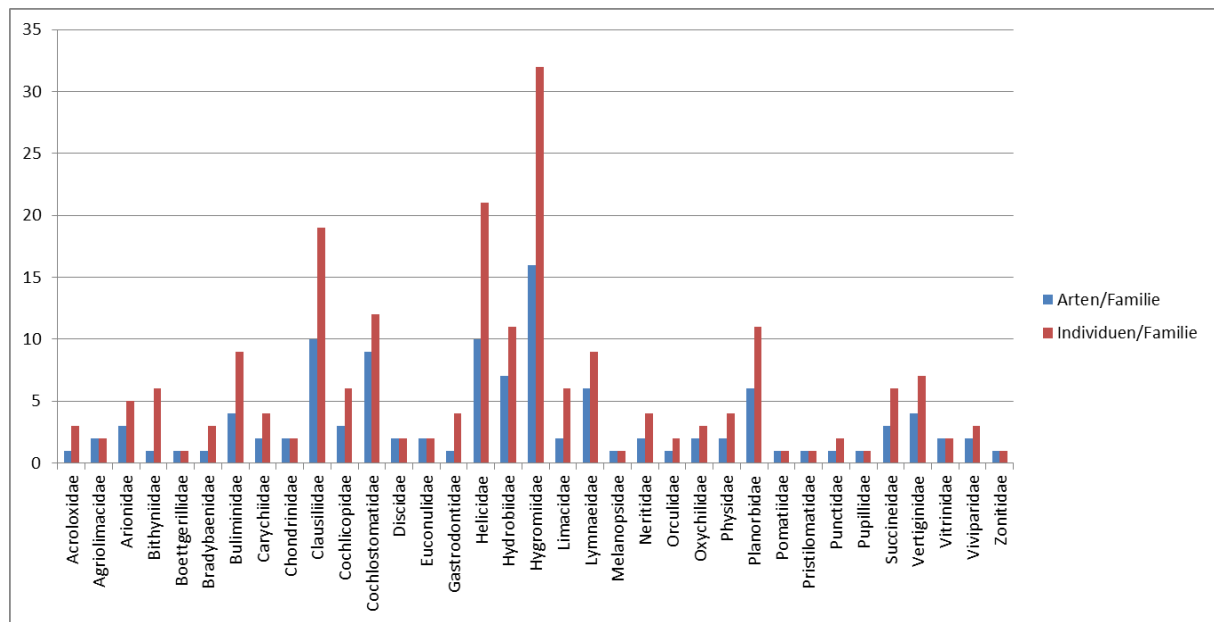
Abbildung 18. Numbers of DNA barcodes obtained from species and individuals per family
