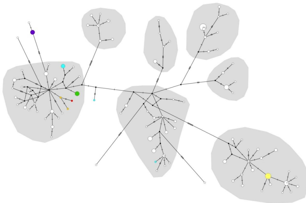
Figure 12. Statistical parsimony network, based on the spacer region between histone H3 and H4 genes of Montenegrina . Sequences / taxa mentioned in the text are highlighted: M. dofleini kastoriae and M. hiltrudae robusta – green; M. fuchsi fuchsi – red; M. rugilabris golikutensis – orange; M. stankovici and M. dofleini pinteri – navy blue; M. perstriata drimica specimens belonging to different mitochondrial haplogroups – yellow; three different sequences from the same M. hiltrudae desaretica specimen – cyan
