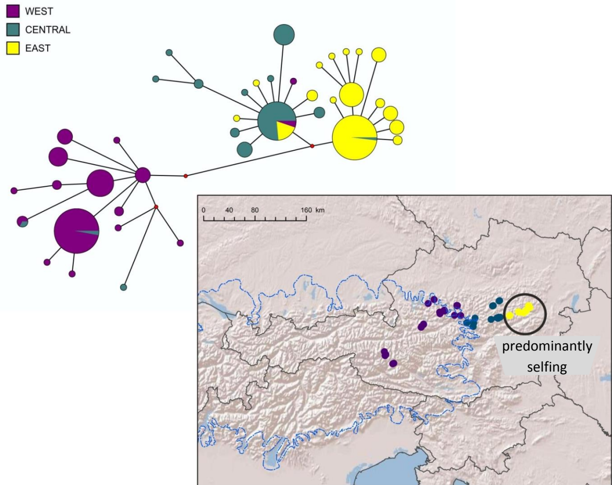
Figure 18. Network showing the three mitochondrial clades of Cyllindrus obtusus and distribution of haplogroups.
